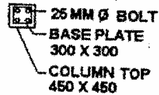
BASE PLATE
