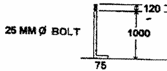
BASE BOLTS
